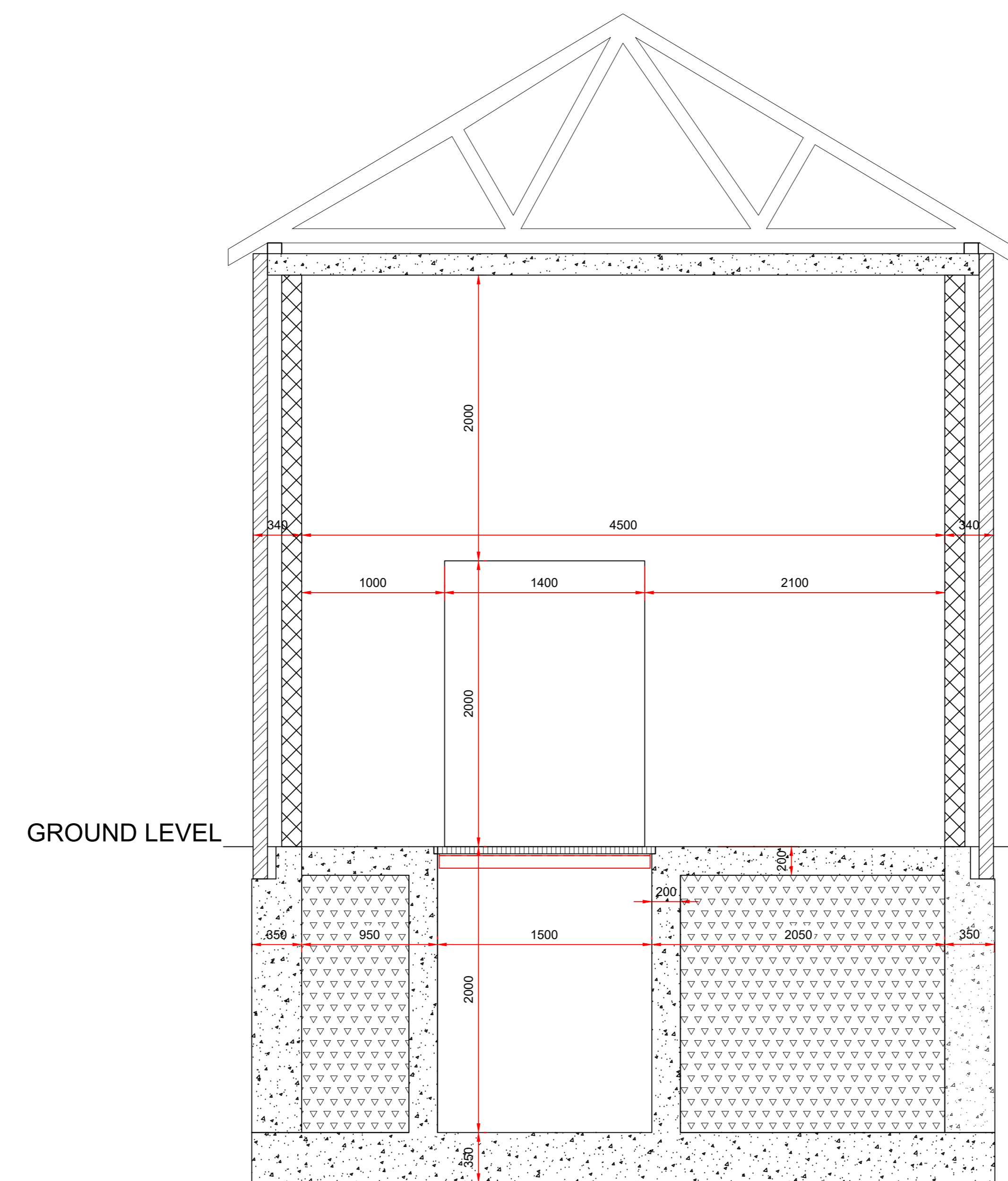
SECTION E-E
