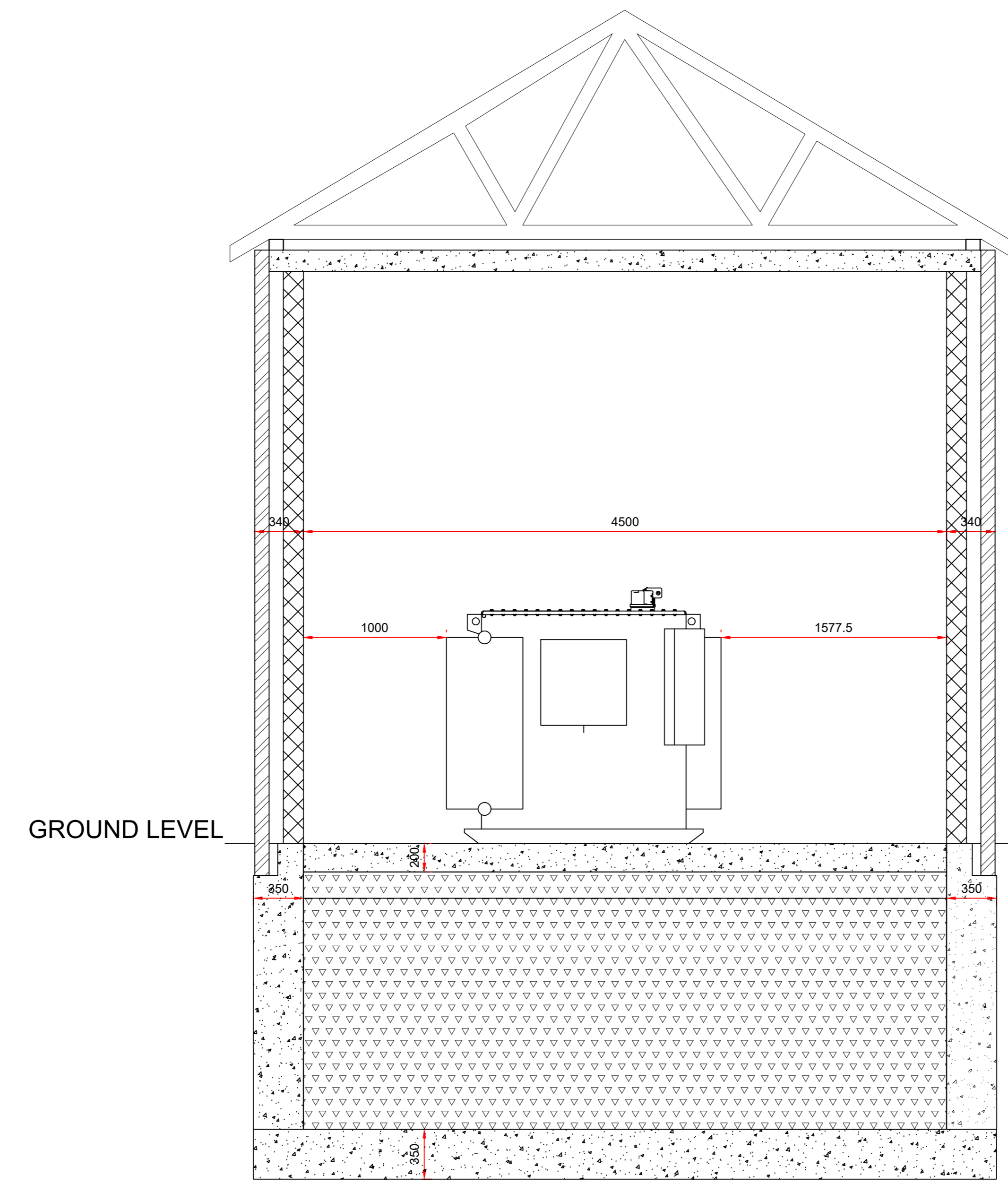
SECTION C-C
