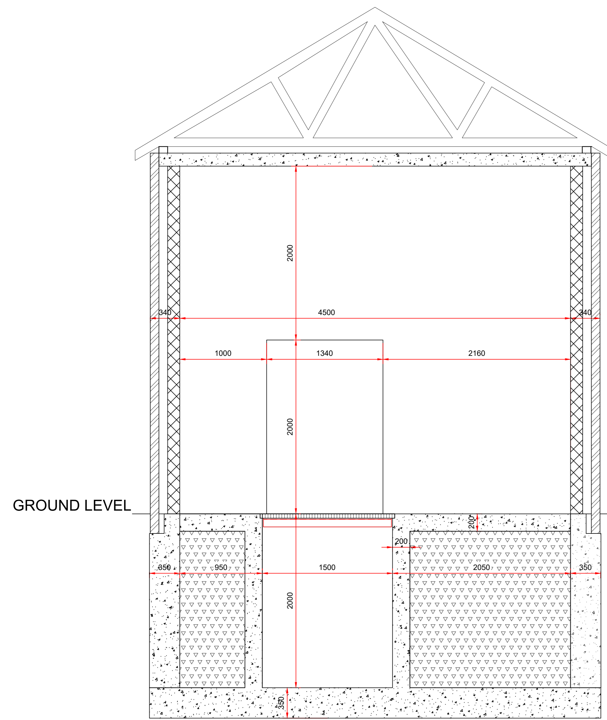
SECTION B-B
